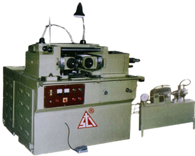
HYDRAULIC THREADING MACHINE
